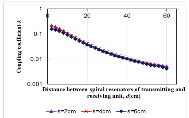
Fig.10 Coupling coefficient k of paired-spiral PP-NN winding direction combination
