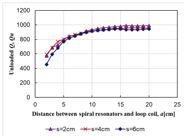
Fig.8 Q_u of paired-spiral PP winding direction for mode 1
