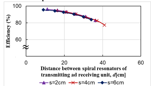
Fig.11 Theoretical value of power transfer energy for paired-spiral PP-NN winding direction combination
