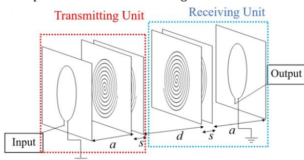
Fig.1 Structure of RC-WPT system using paired-spiral resonators.
