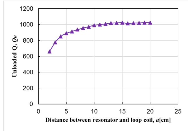
Fig.6 Q_u of paired-spiral with same winding direction (PP or NN)
