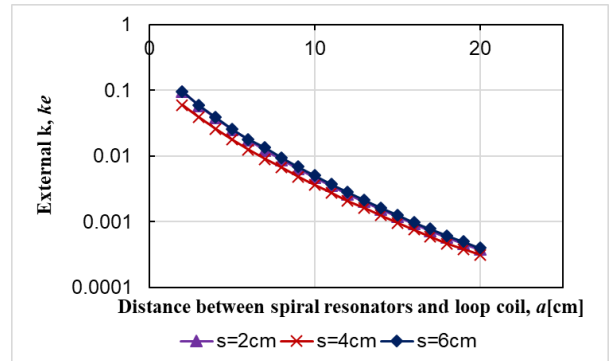
Fig.9 k_e of paired-spiral PP winding direction for mode 1
