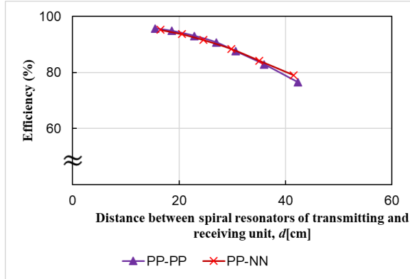
Fig.7 Experimental value of power transfer energy for PP-PP and PP-NN combination when s=2\text{cm}
