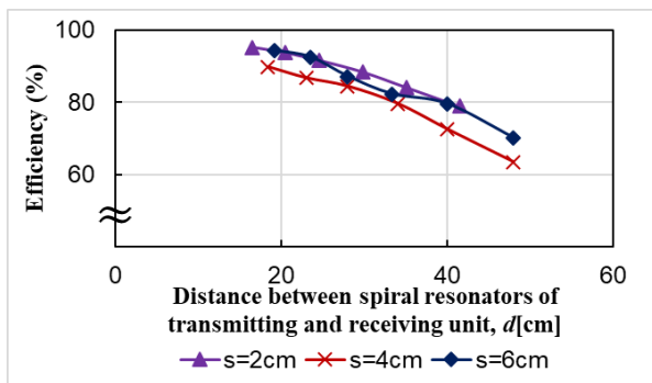
Fig.12 Experimental value of power transfer energy for paired-spiral PP-NN winding direction combination
