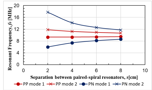
Fig.5 Resonant frequency f_0 for resonators with PP and PN winding direction when a=14\text{cm}
