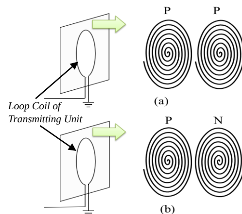
Fig.3 Example setup for paired-spiral resonators with PP or PN winding direction
