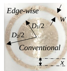
Fig.2 Dual-Spiral Resonator
