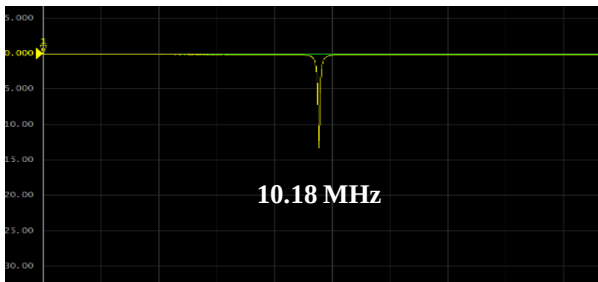
←Low frequency High frequency→ (b) Grounded-Loop Spiral Resonator
