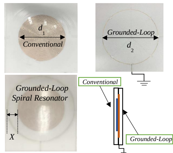
Fig.3 Schematic setup for grounded-loop spiral resonator
