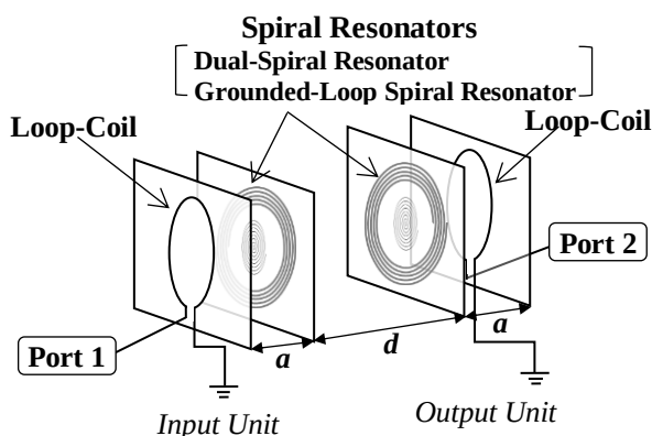
Fig.1 Schematic setup of RC-WPT system
