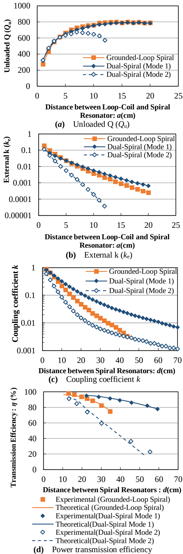
Fig.4 Measured with the Grounded-Loop Spiral Resonator and the Dual-Spiral Resonator
